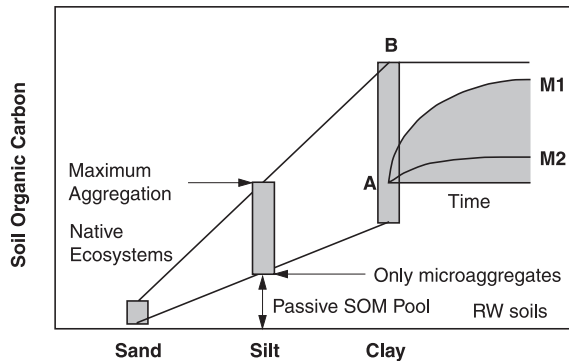
Figure 2. Conceptual model for soil organic carbon.
