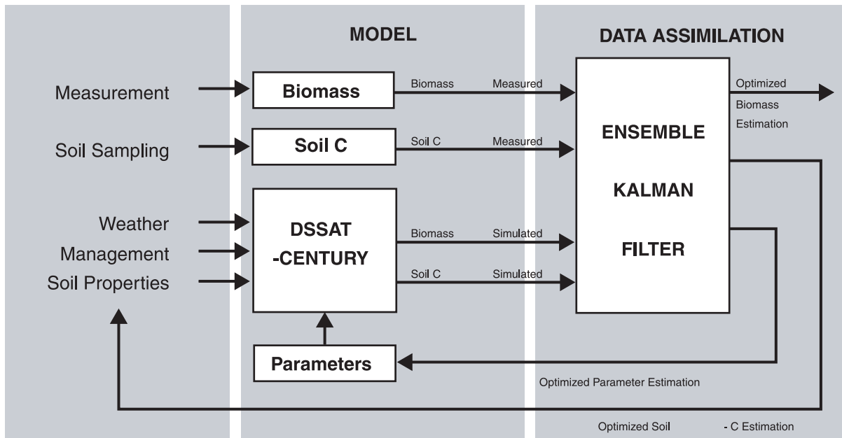
Figure 1. Schematic showing optimal soil C estimates using the EnKF to integrate observed soil C and biomass data with predictions of soil C using the DSSAT-CENTURY model (from Koo et al. , 2003).
